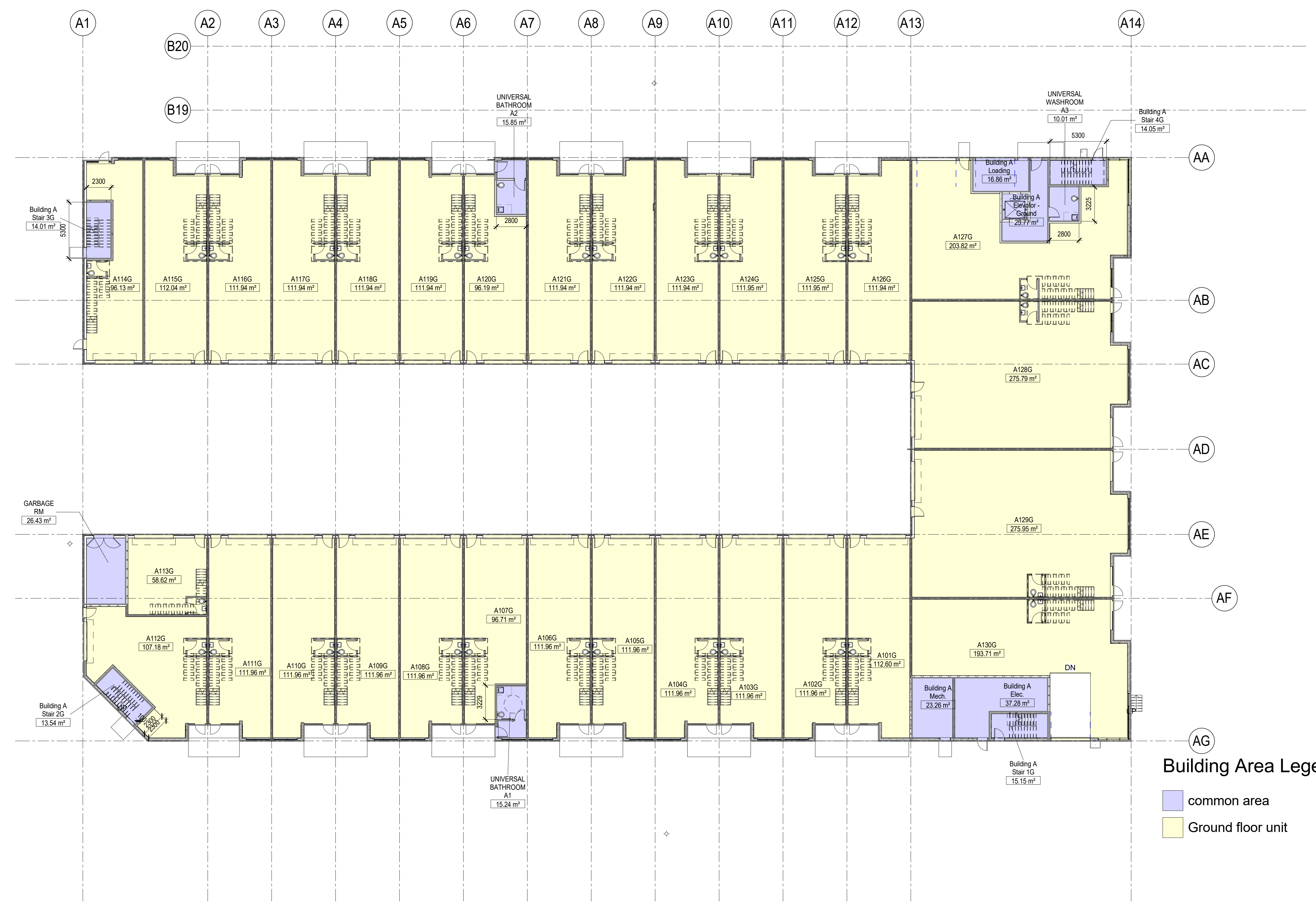
Building A Ground Floor
